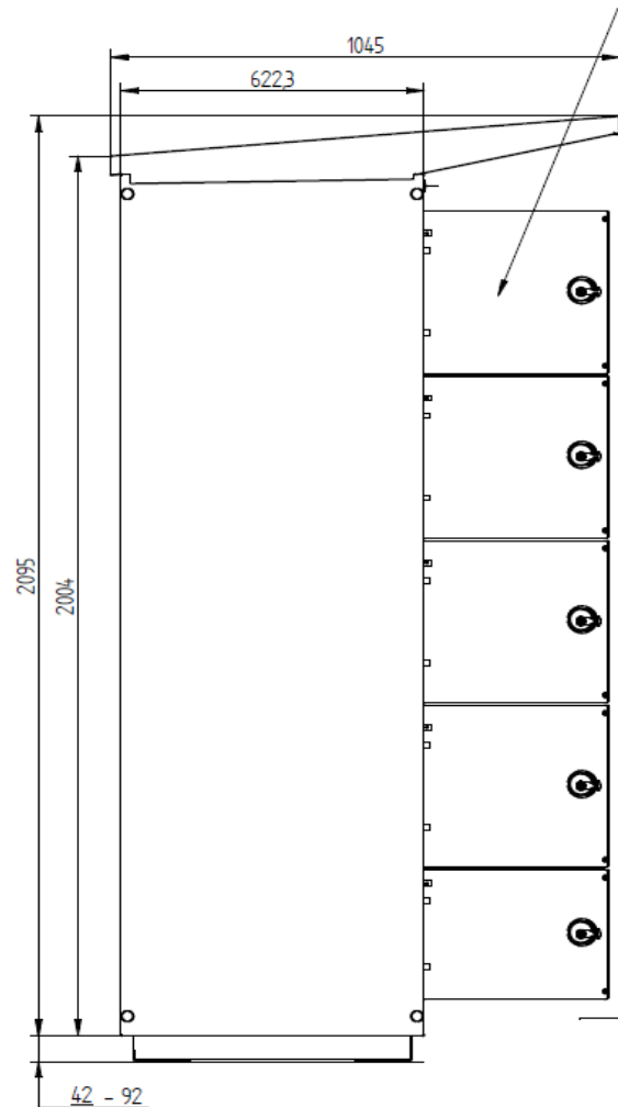
2) Side view with roof structure, open doors:
